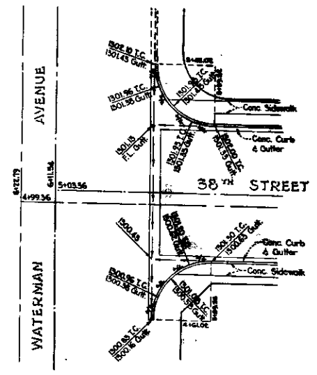
INTERSECTION DETAIL STREET & WATERMAN AVENUE SCALE 1"=20'
