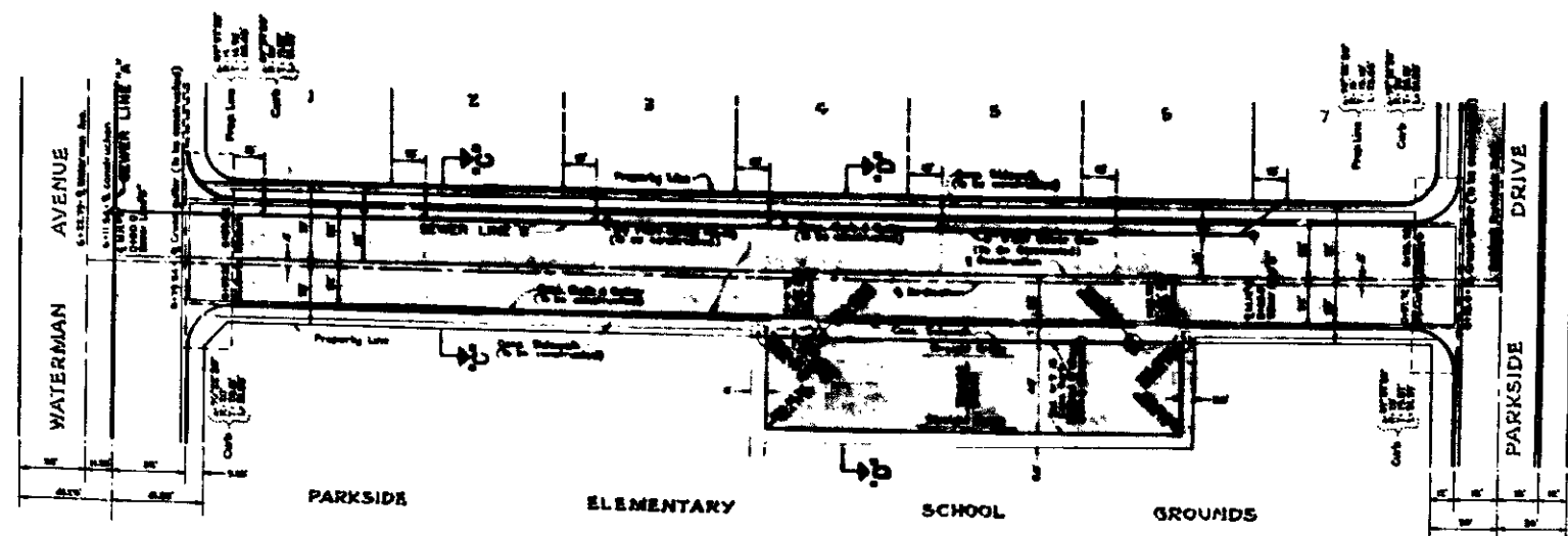
PLAN - 38 TH STREET SCALE 1"=40'
